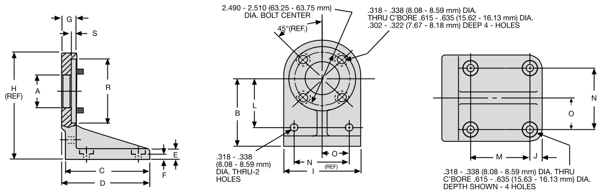
37892-1 FOOT MOUNTING BRACKET
