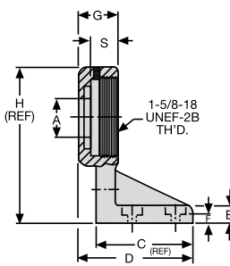
37894 FOOT MOUNTING BRACKET
