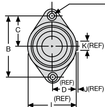
.193 - .213 (4.90 - 5.41 mm) DIA. THRU C'BORE .365 - .385 (9.27 - 9.78 mm) DIA. DEPTH SHOWN - 2 HOLES
