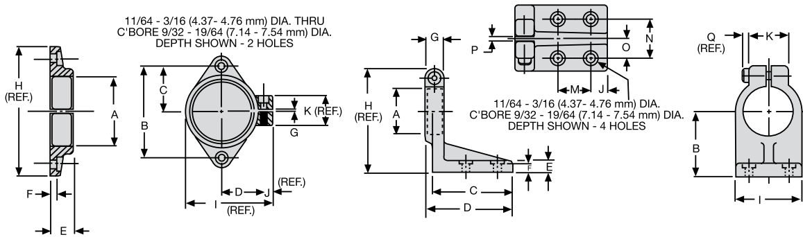
41058 FLANGE MOUNTING BRACKET
