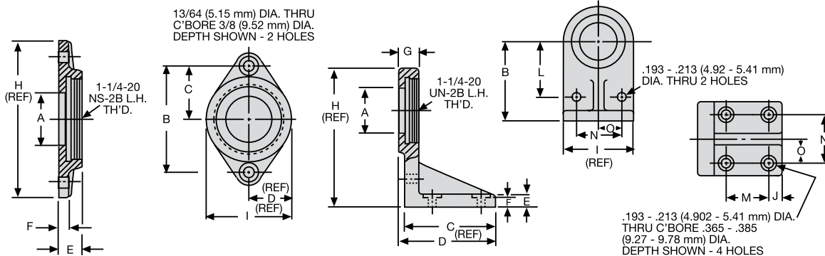
37898 FLANGE MOUNTING BRACKET
